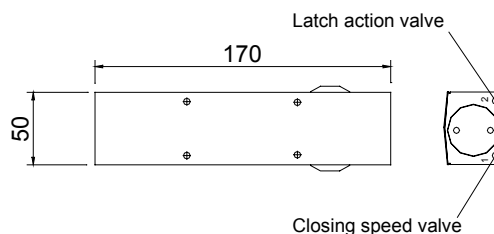
TS1500 BODY
